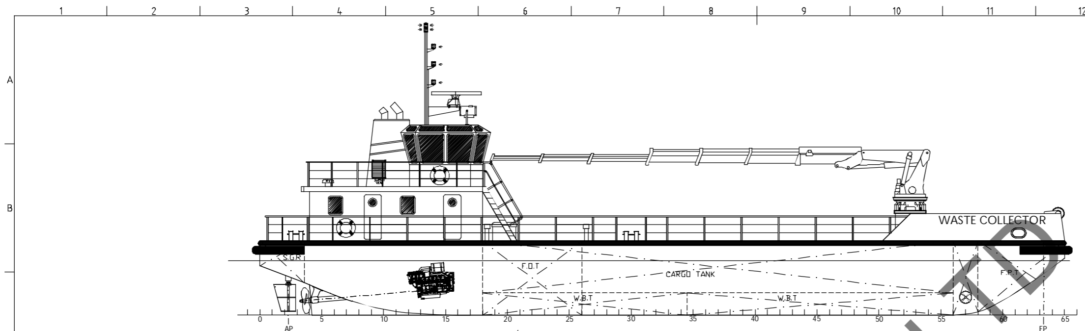
PROFILE
