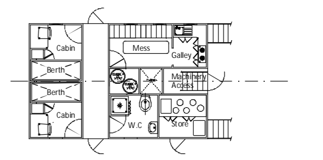
DECK HOUSE
